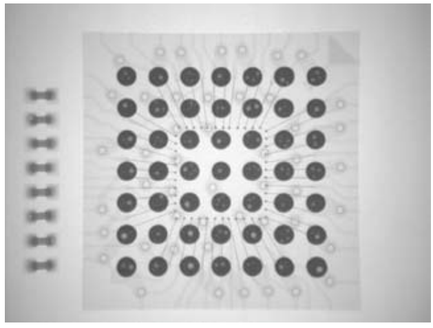
BGA X-ray Inspection
